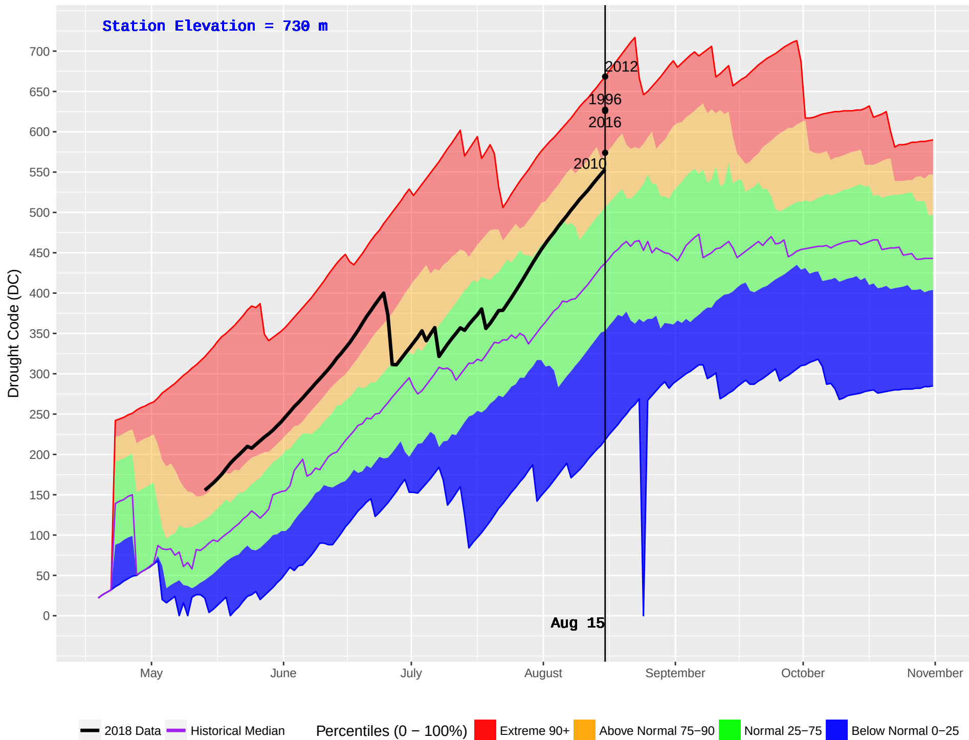
BOYA LAKE (445) : Historical (1985–2016) and Current (2018) Daily Drought Code (DC)
