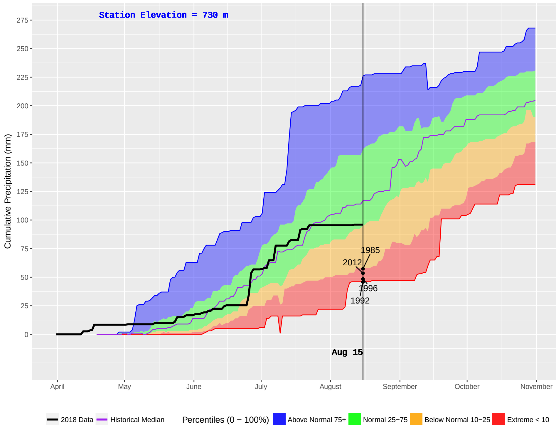
BOYA LAKE (445) : Historical (1985–2016) and Current (2018) Daily Cumulative Precipitation
