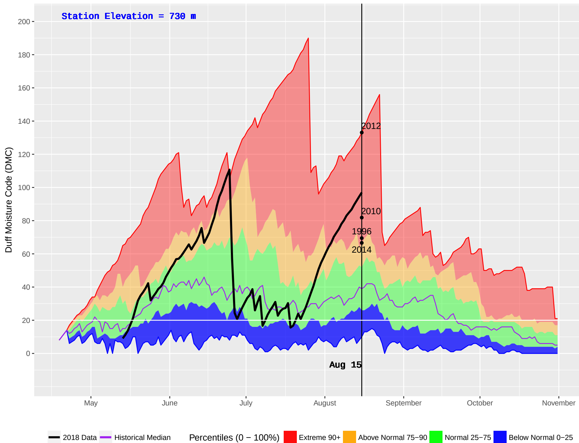
BOYA LAKE (445) : Historical (1985–2016) and Current (2018) Daily Duff Moisture Code (DMC)
